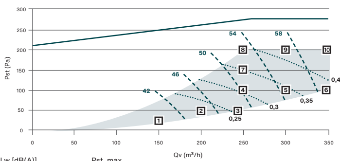
ComfoAir Flex 350
