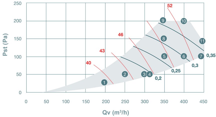
Zehnder ComfoAir Q450 ST
